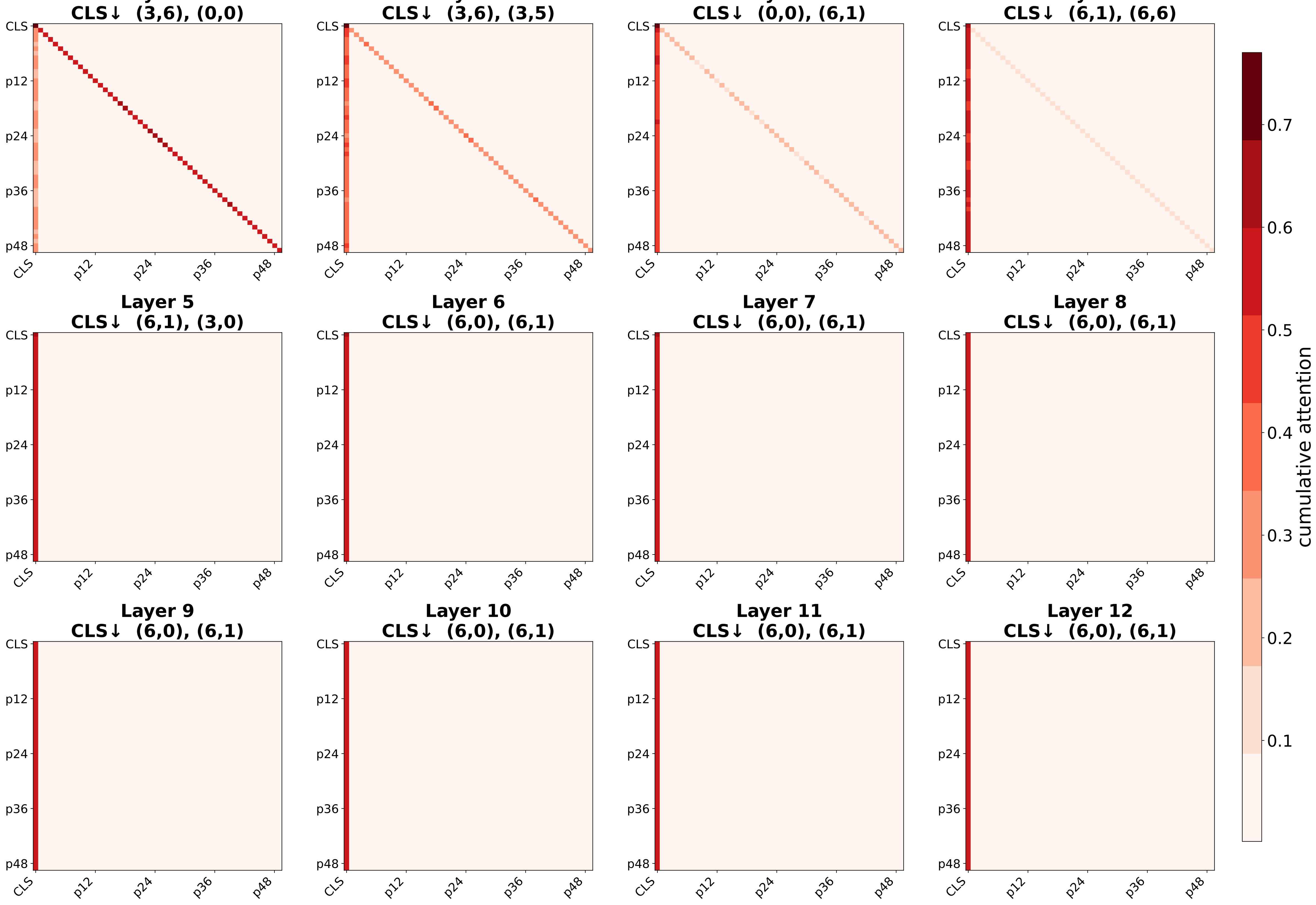
16 — heads-averaged — Cumulative attention rollout matrix per layer (50×50: 1 CLS + 7×7 patches)
