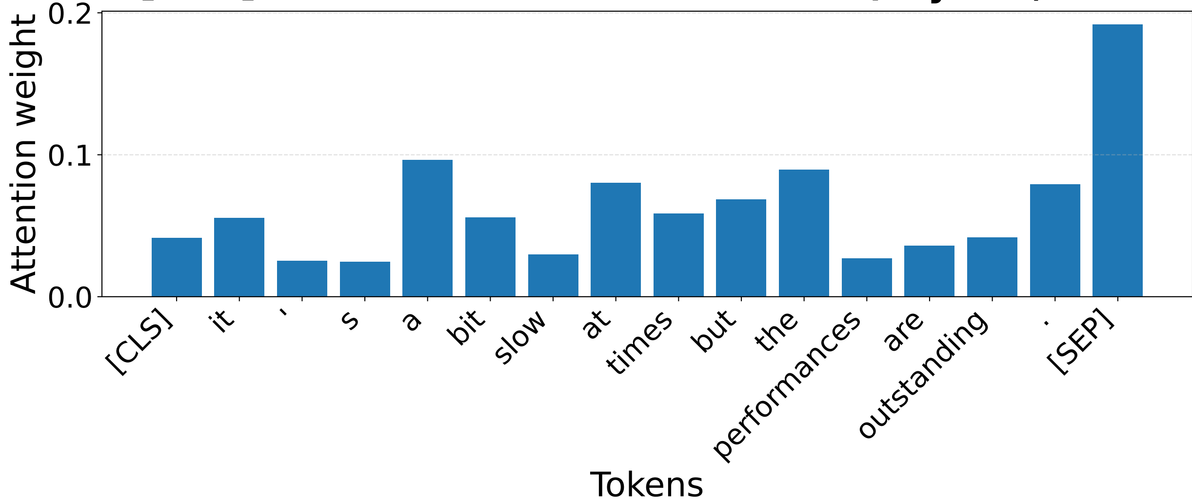
S3 [POS] – Vanilla attention CLS row (Layer 1, Head 1)
