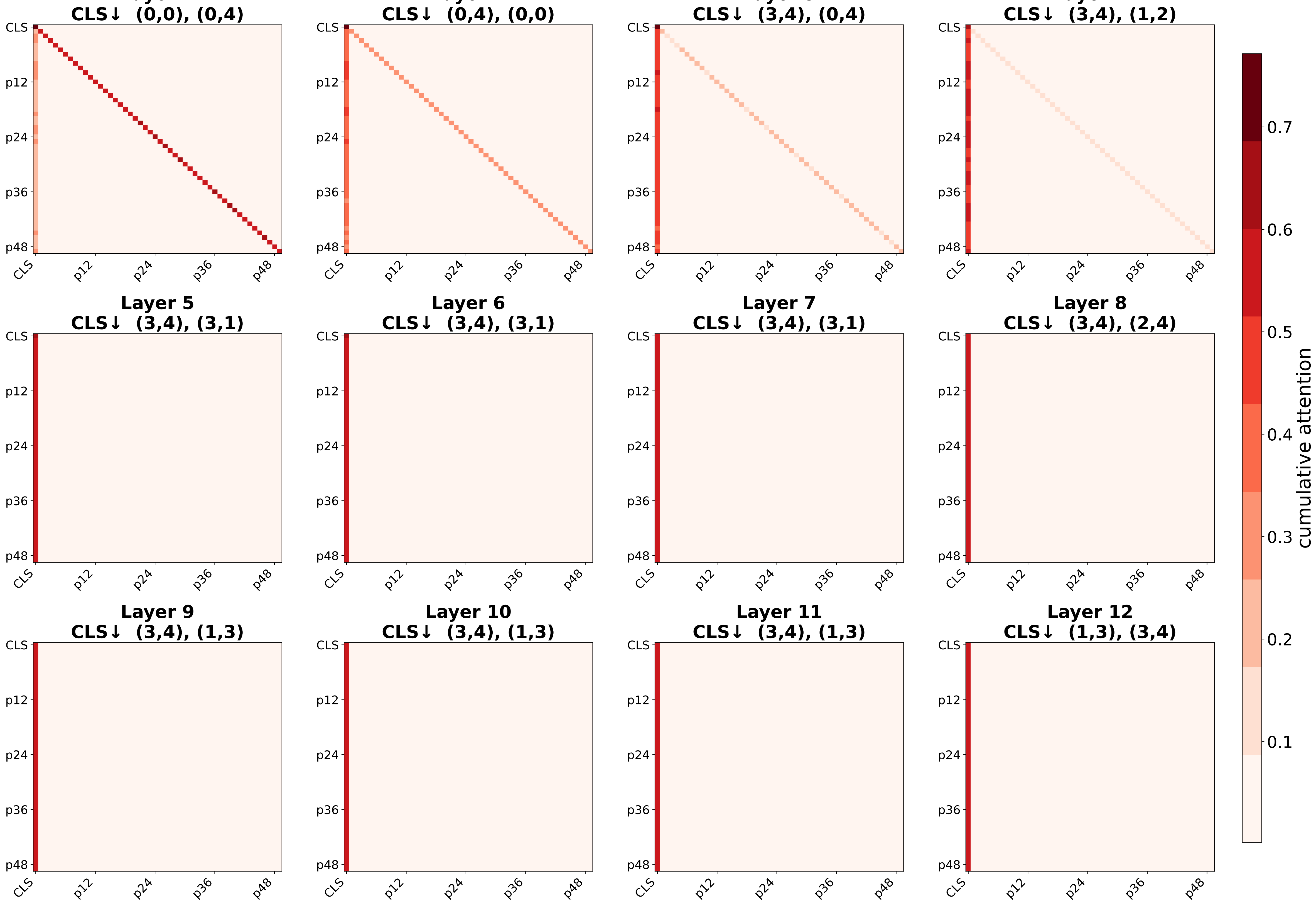
I1 — heads-averaged — Cumulative attention rollout matrix per layer (50×50: 1 CLS + 7×7 patches)
