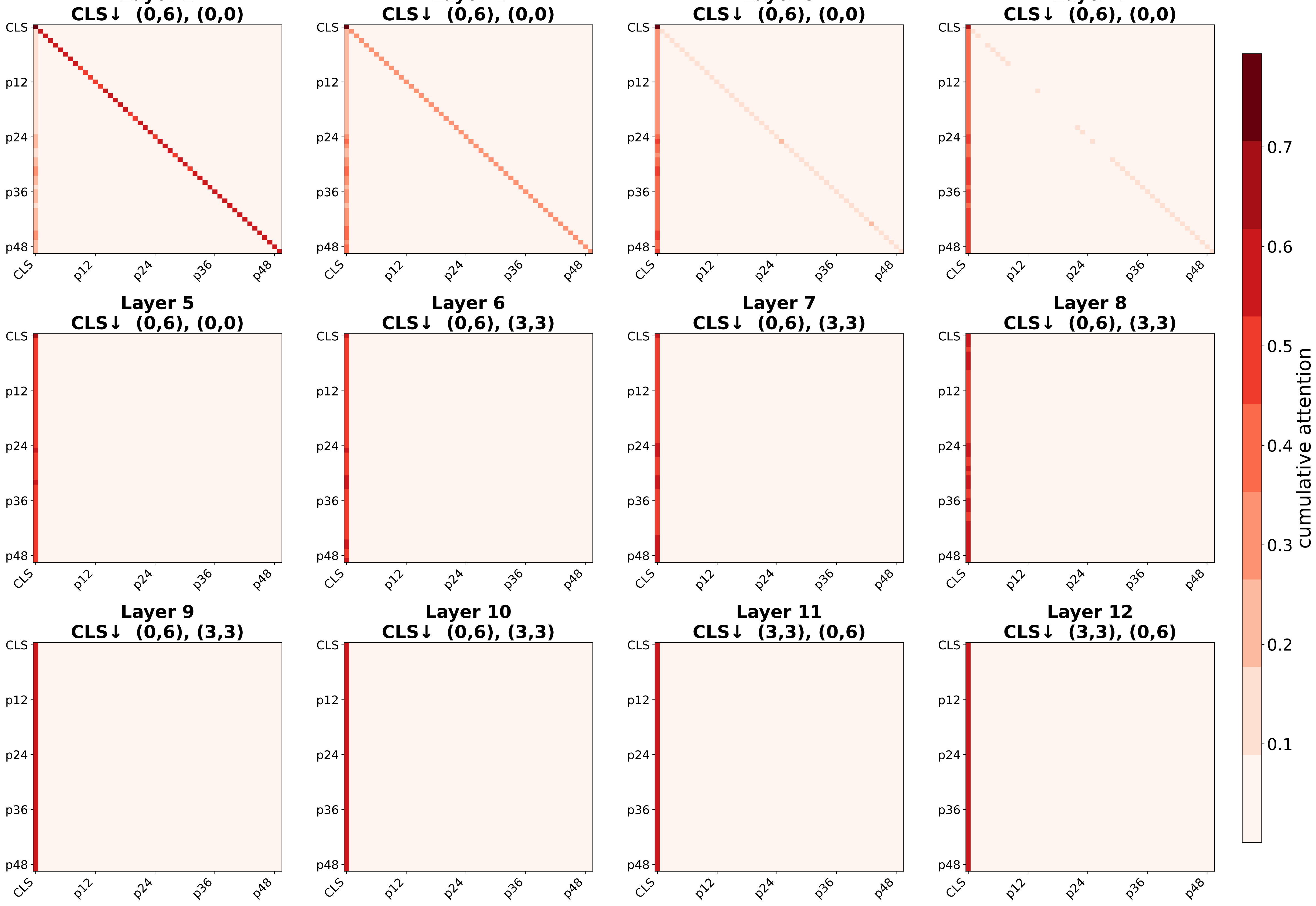
14 — heads-averaged — Cumulative attention rollout matrix per layer (50×50: 1 CLS + 7×7 patches)
