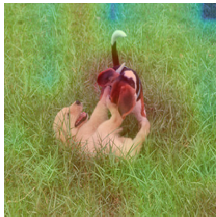
Head 10
