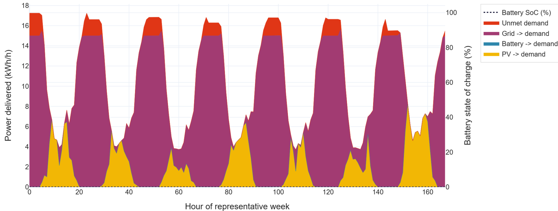
Hourly smart-charging dispatch — PV / battery / grid (Theme 2)
