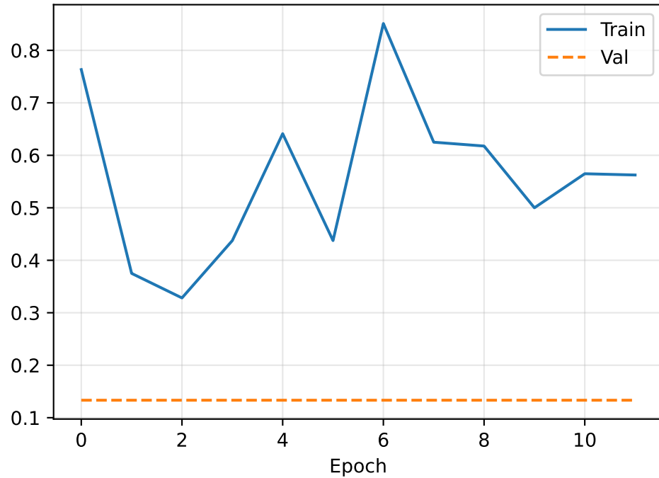
EfficientNetB0 — Accuracy
