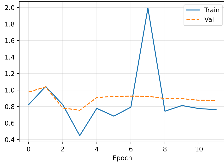
EfficientNetB0 — Loss
