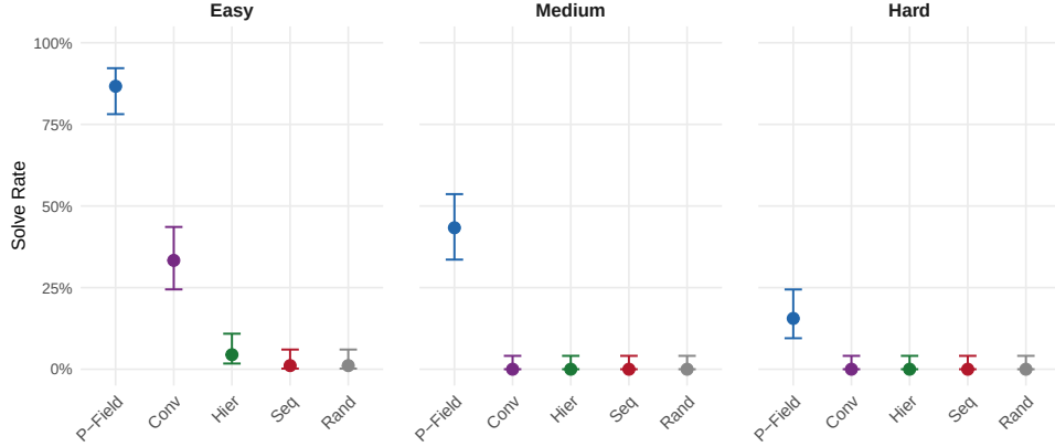
Fig. 1 Strategy comparison by difficulty level. Error bars show 95% Wilson Confidence Intervals. Pressure-field outperforms all baselines at every difficulty level. On medium and hard problems, only pressure-field achieves non-zero solve rates.
