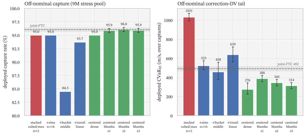
Figure 17: Objective-centering under the high-dispersion stress probe (9M pool, shared noise path). Left: deployed capture rate; right: deployed correction-DV \text{CVaR}_{95} over captured runs. The five dense lever cells are n = 1000 ; the three centered-Mamba seeds and the retrained joint-FTC reference (dashed line, shaded interval) are the n = 10,000 cells of Table 6; whiskers are bootstrap 95% intervals where the data carry them. The medium-regime stack (red) carries an enormous tail; centering recovers it (green) and transfers to the Mamba, beating the retrained joint-FTC. The central bucket alone trades capture for the tail (left, 84.5%), so the three levers are read together. Capture and tail are shown separately because the levers trade them off.
