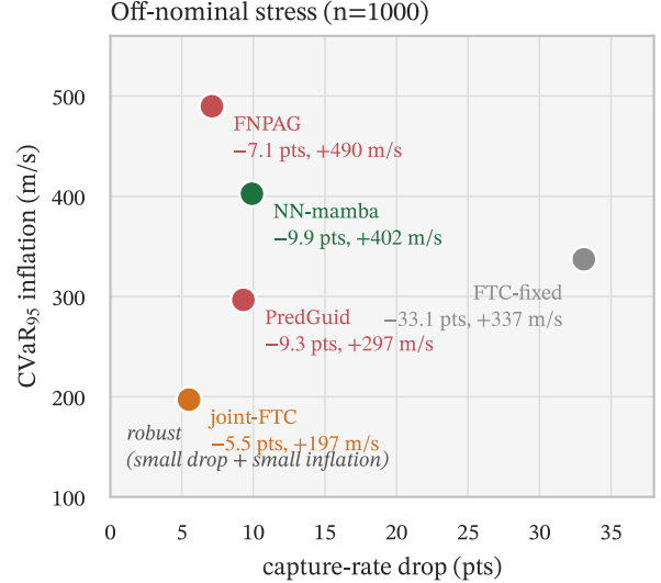
Figure 15: Off-nominal stress. The analytic joint-FTC is the most robust to distribution shift; the medium-trained network generalizes less well, the paper’s robustness caveat.
