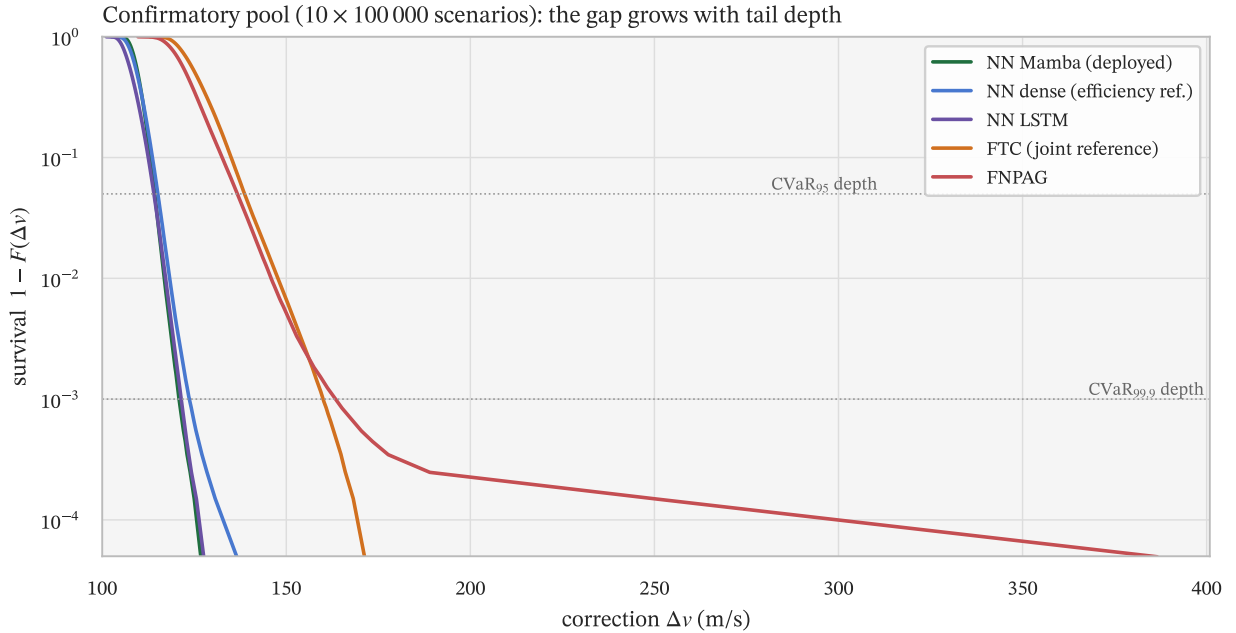
Figure 16: Empirical survival curves of the correction \Delta v on the confirmatory sizing pool ( 10 \times 100,000 scenarios) per scheme; log scale, curves subsampled every \approx 100 th order statistic). The network-to-classical separation grows with tail depth – the sizing thesis in one picture.
