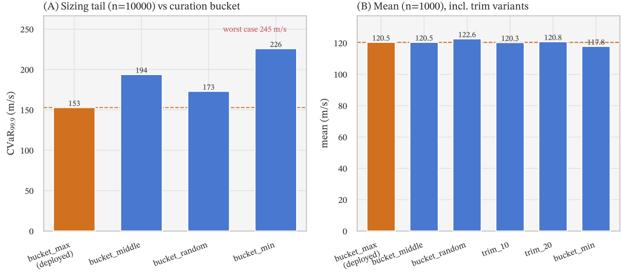
Figure 5: Seed curation. Left: far-tail \text{CVaR}_{99.9} ( n = 10,000 ) per curation bucket – selecting the hardest seed per cost-CDF bin (the “max” bucket) compresses the sizing tail, and the easiest-seed bucket blows it up (worst case 245 m/s). Right: mean ( n = 1000 ) – the easiest bucket wins the mean, the optimize-the-average trap; the trim variants match the max bucket and were not carried to the far-tail pool.
