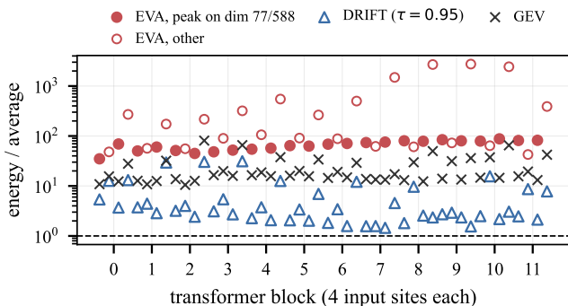
Fig. 1. Input energy along each module’s leading initial direction, relative to an average direction (log scale; RoBERTa-base, ChemProt). One point per input site: W_Q , W_K and W_V read the same block input. Filled: EVA’s leading direction peaks on outlier dimension 77 or 588; hollow circles: the attention-output and feed-forward hidden inputs, which are not in the hidden-state basis. Open triangles: DRIFT after deflation; crosses: GEV.
