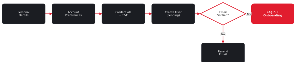
Figure 4 — Registration and onboarding flow.
