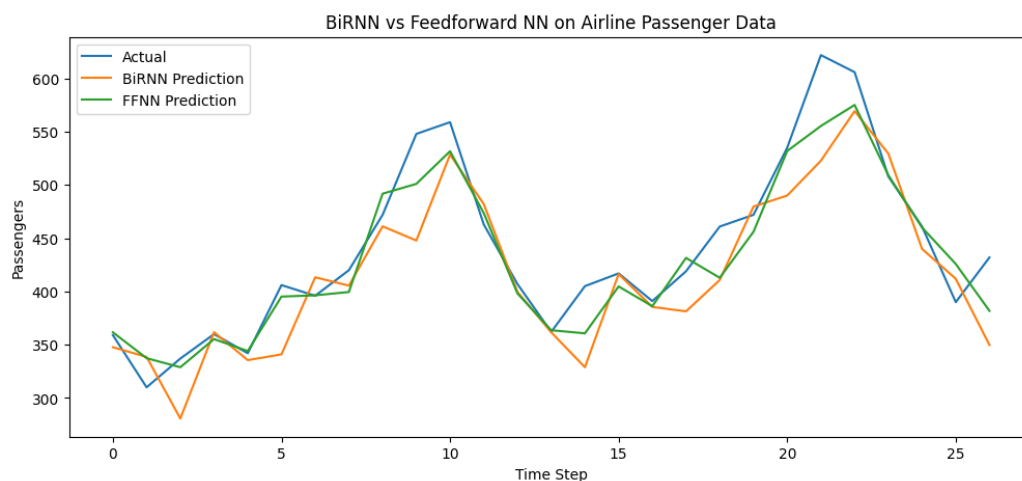
BiRNN vs Feed-forward NN on the Airline Passenger data
