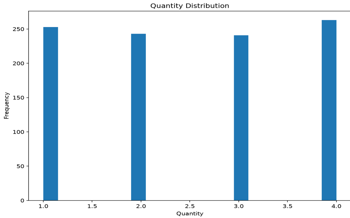
Quantity Distribution
