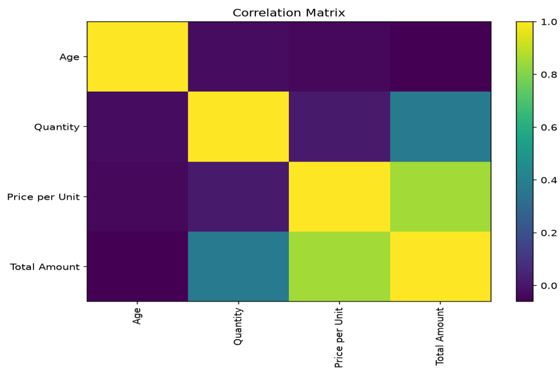
Correlation Matrix
