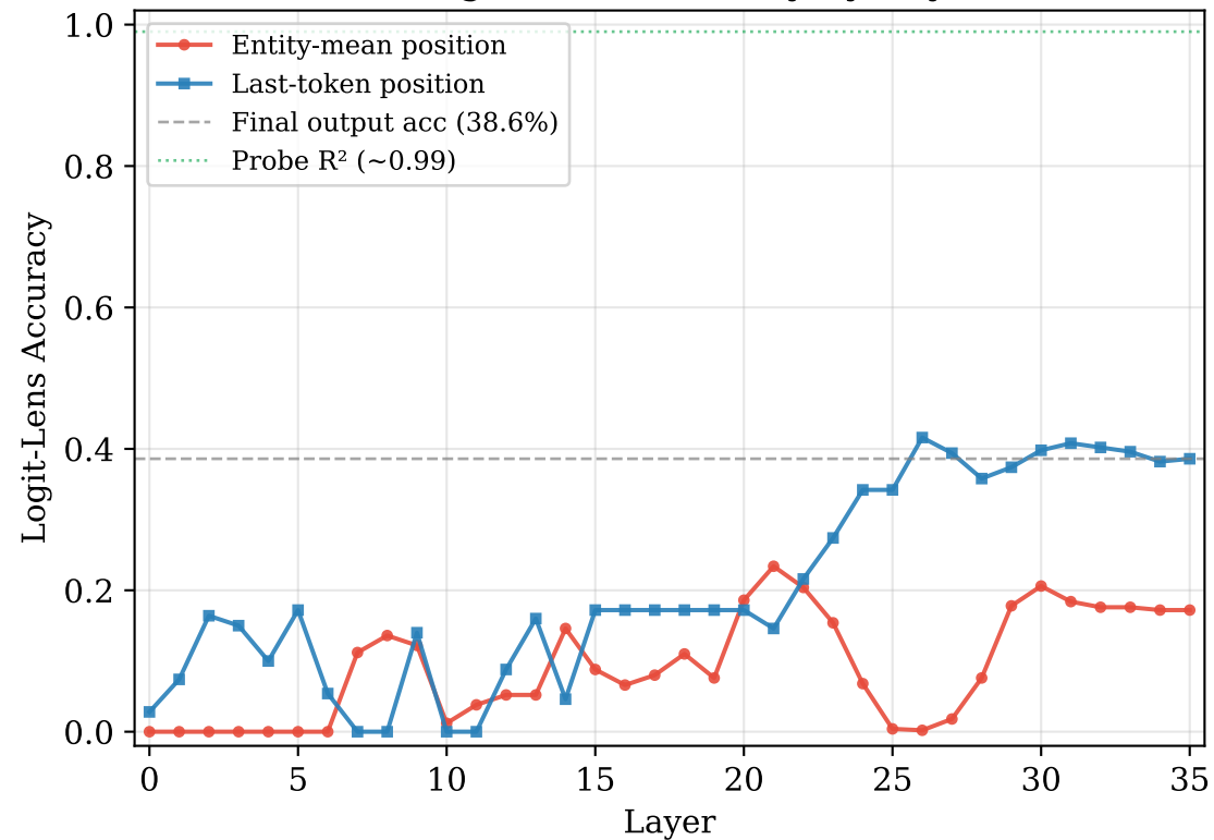
(a) Logit-Lens Accuracy by Layer
