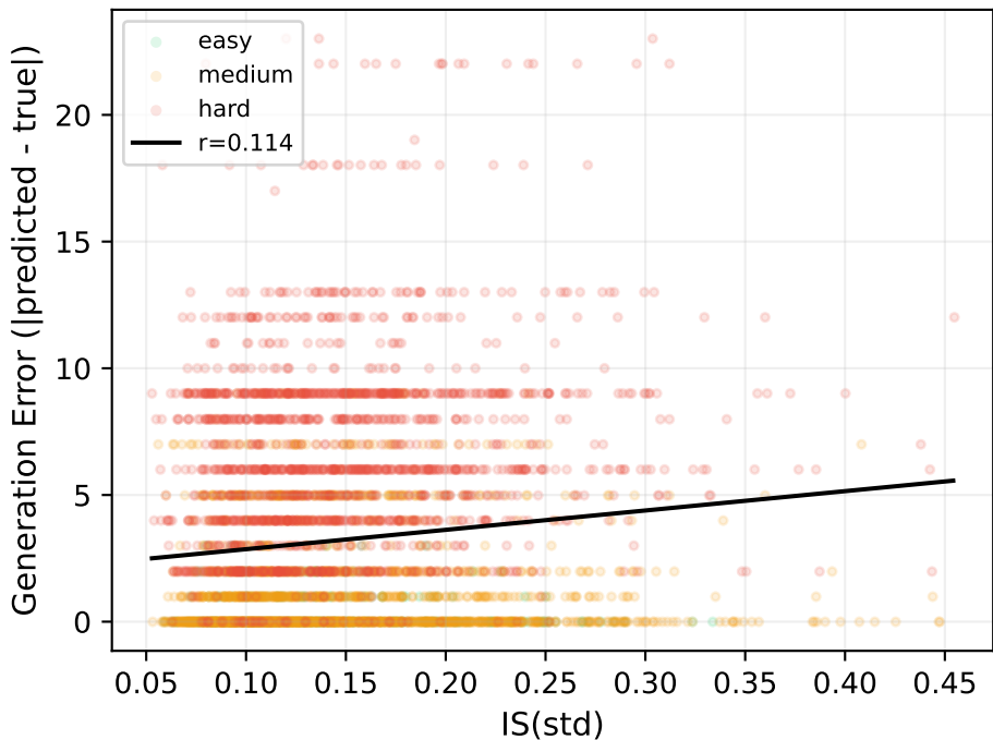
IS vs Generation Error (Qwen3-8B, matched setting)
