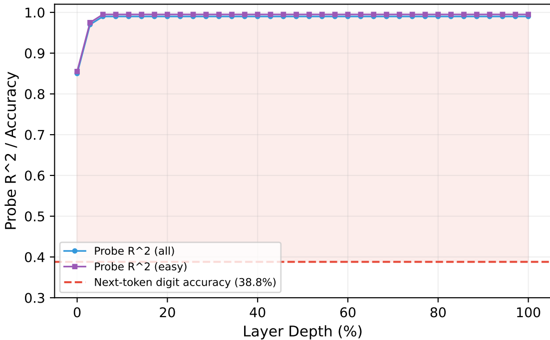
Representation-Output Gap (Qwen3-8B)
