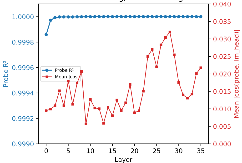
Near-Perfect Encoding, Near-Zero Alignment
