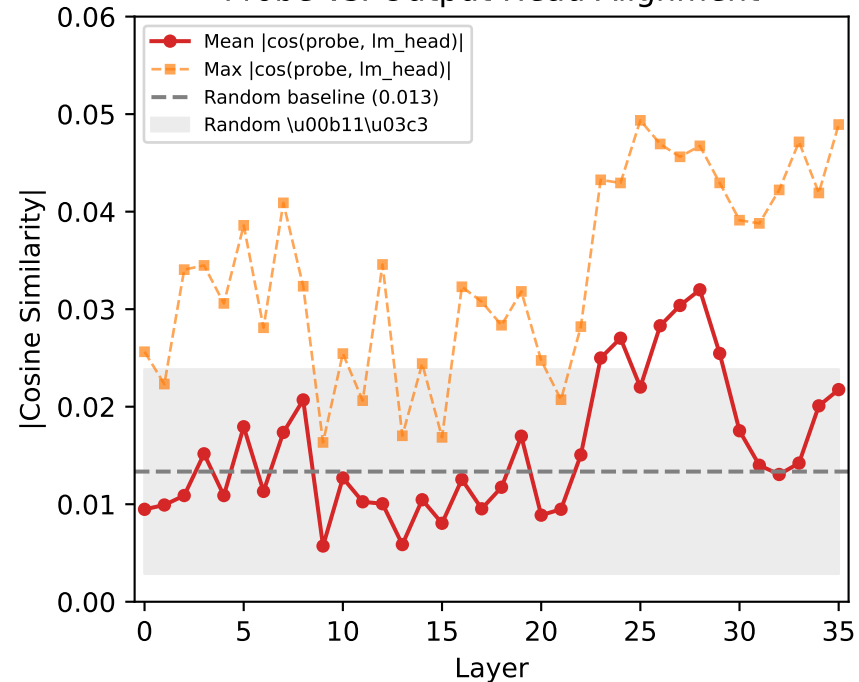
Probe vs. Output Head Alignment
