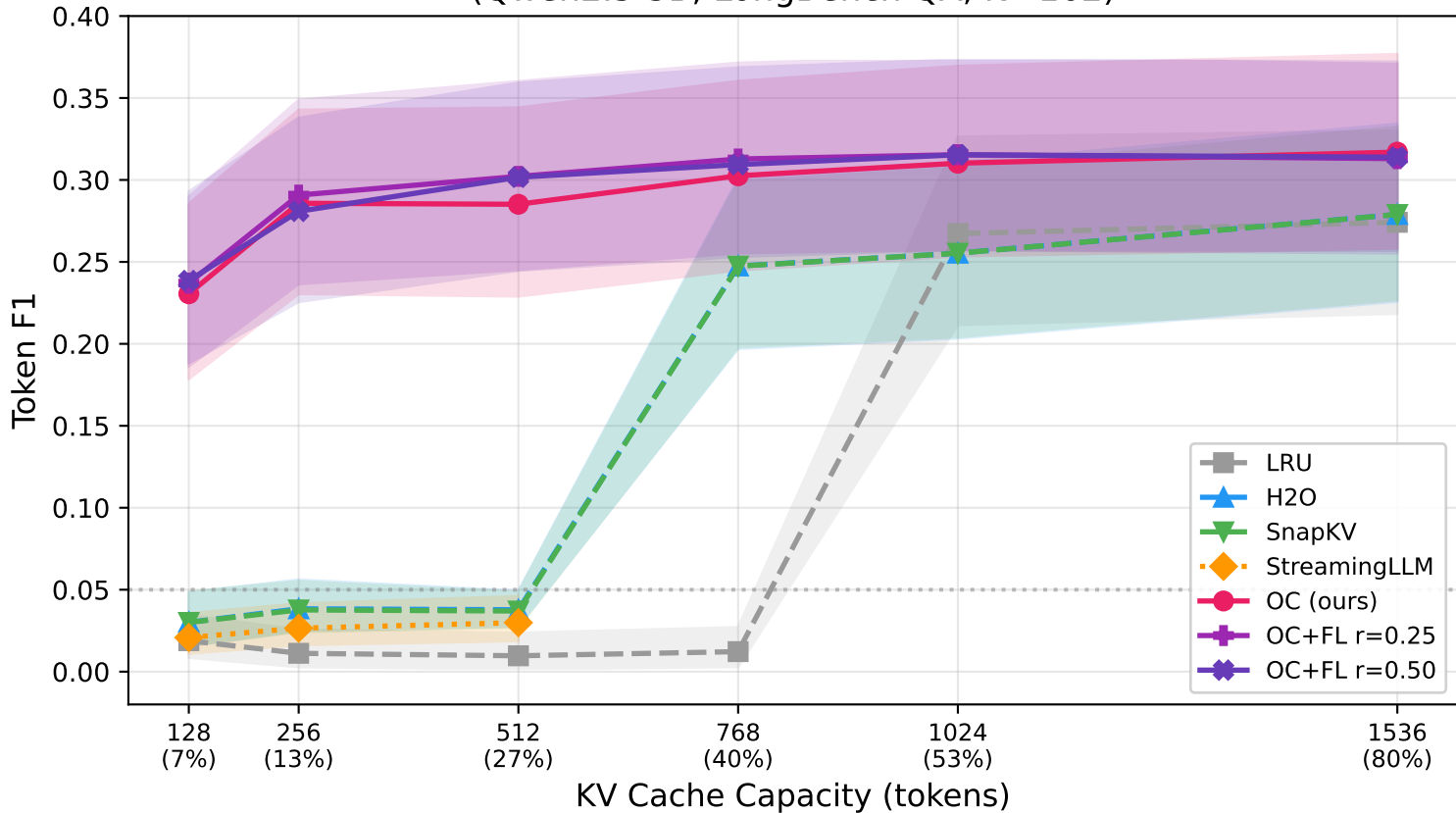
KV Cache Eviction: Quality vs. Capacity (Qwen2.5-3B, LongBench QA, N=162)
