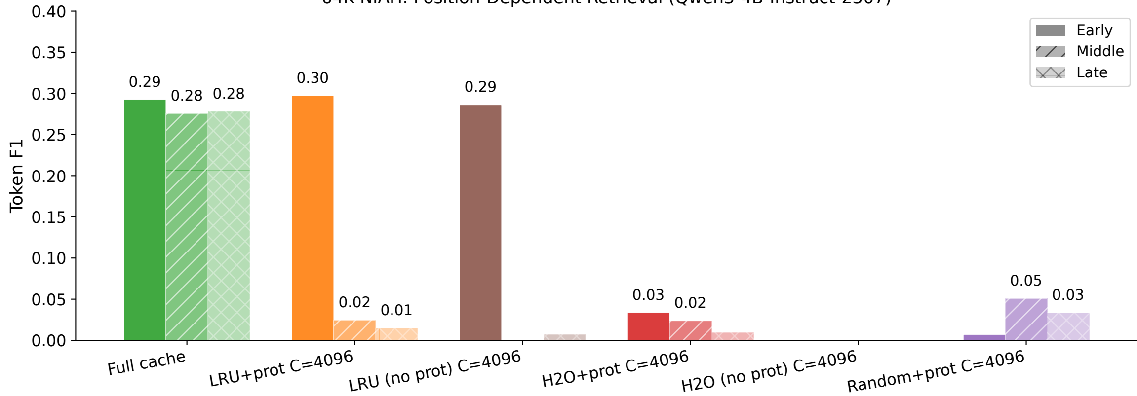
64K NIAH: Position-Dependent Retrieval (Qwen3-4B-Instruct-2507)
