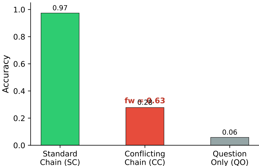
Conflicting-Answer Experiment (Qwen 2.5-3B, N=500)
