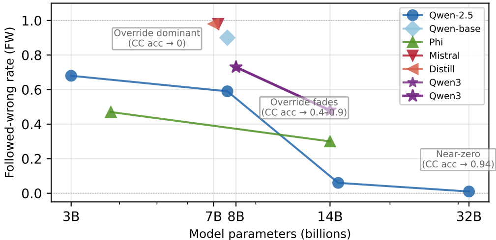
Answer-text override attenuates with model scale
