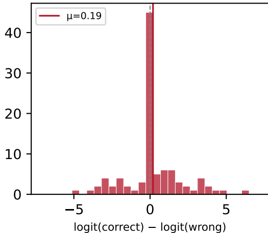
Conflicting chain (wrong suffix) wrong > correct in 23%
