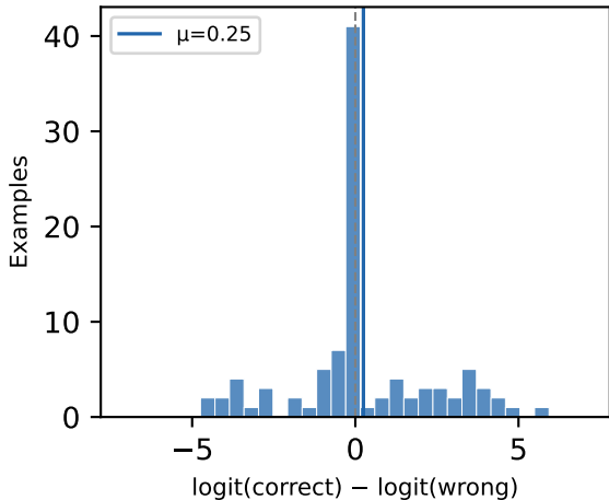
Standard chain (correct suffix) correct > wrong in 31%
