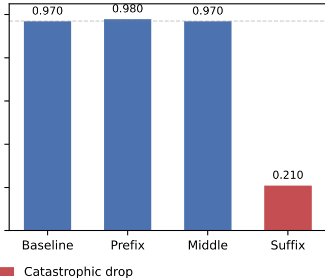
GSM8K-v1: answer in suffix
