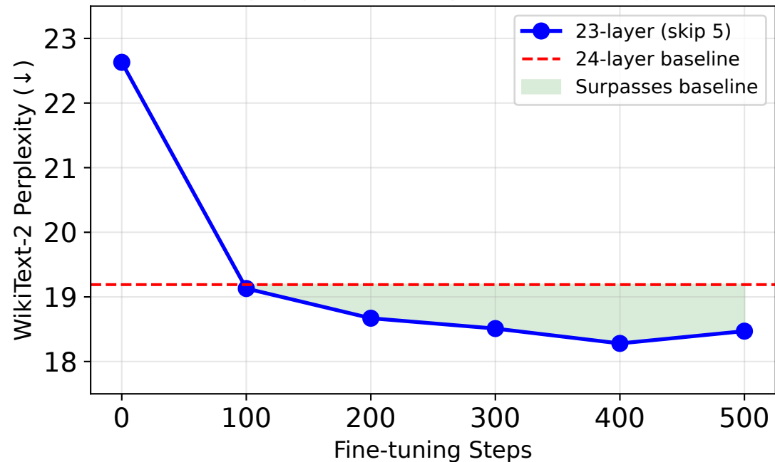
Skip-Layer Recovery via Fine-tuning
