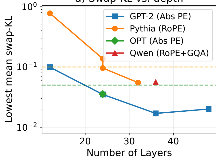
a) Swap-KL vs. depth
