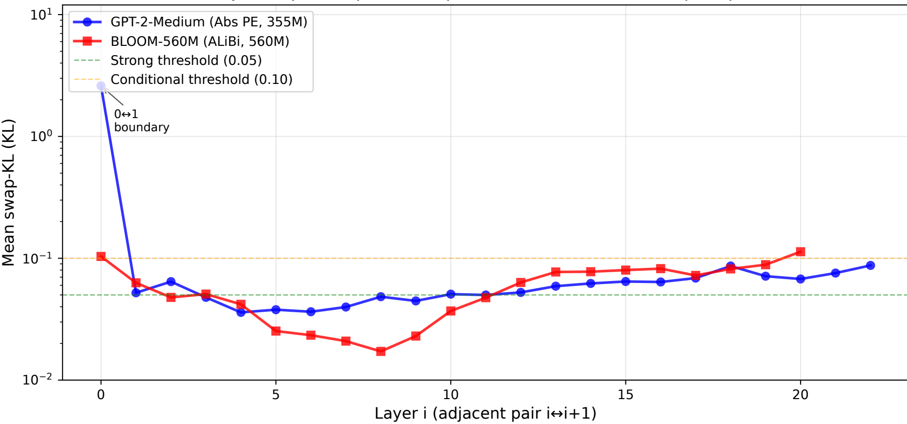
Adjacent-pair empirical swap-KL: GPT-2 vs BLOOM (100 prompts)
