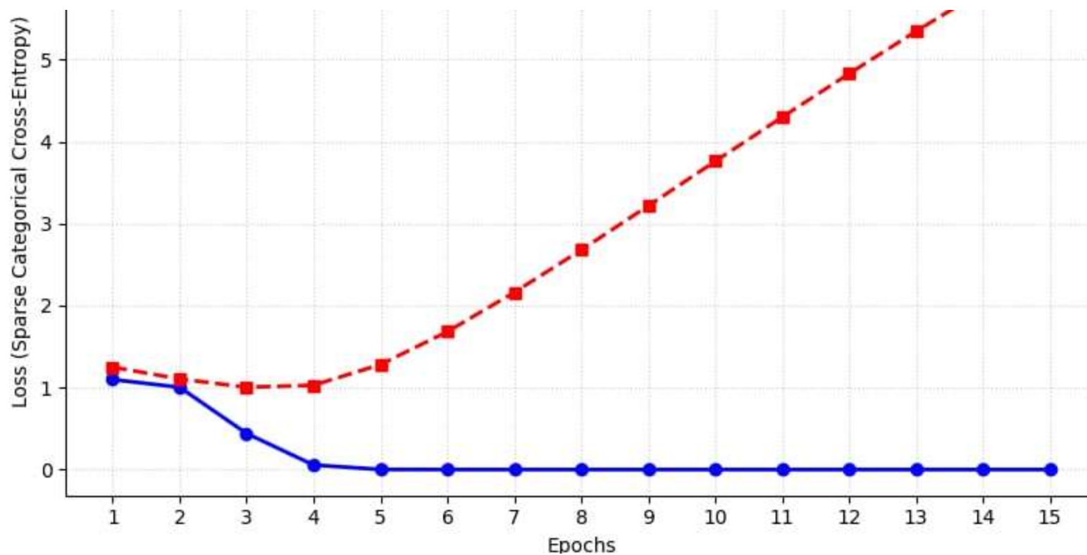
Performance Monitoring: Loss Curves (EXP-04)
