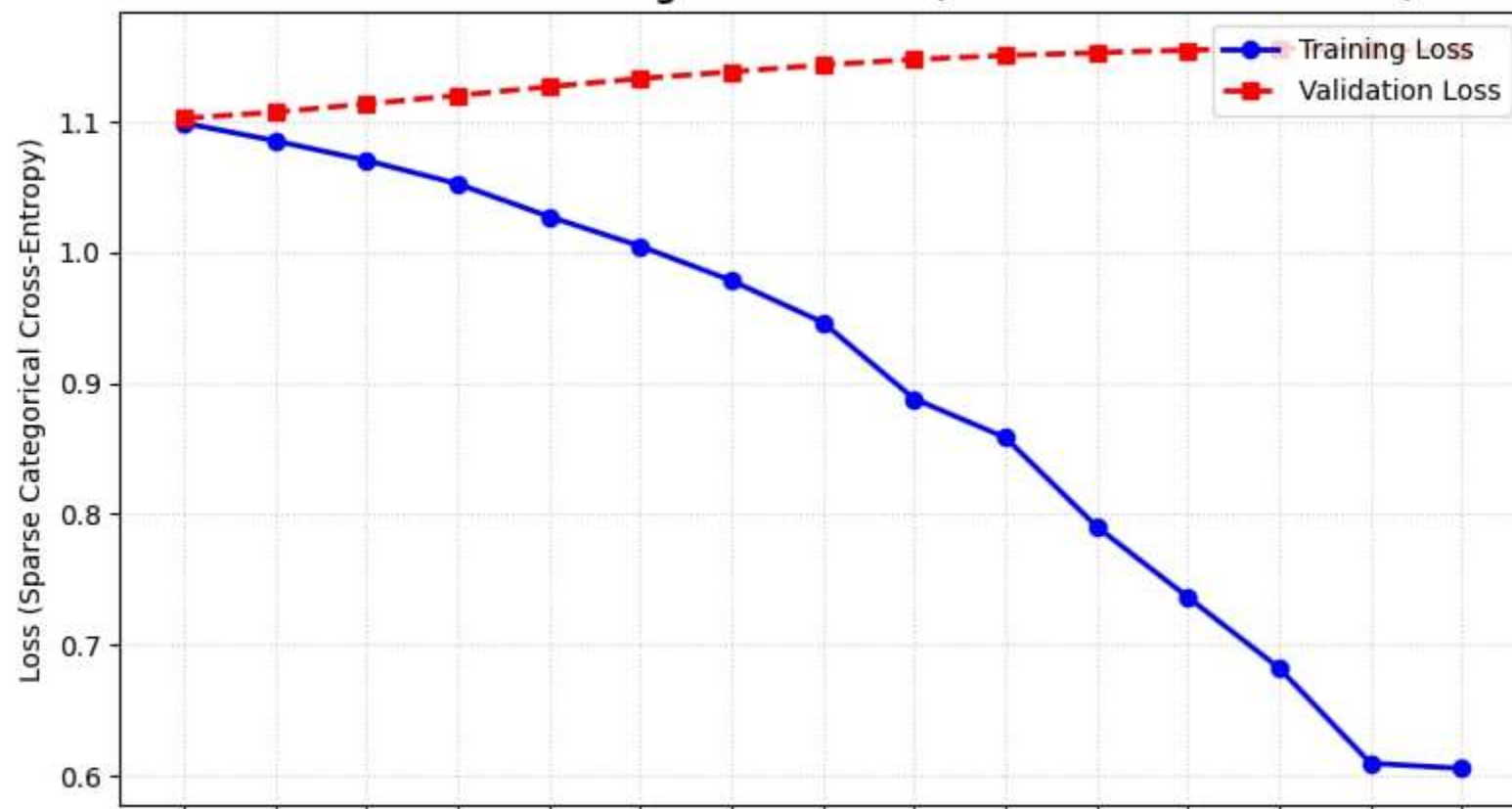
Performance Monitoring: Loss Curves (EXP-01-KERAS-BASELINE)
