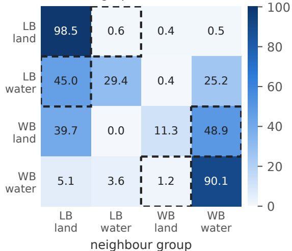
Raw CLIP graph
