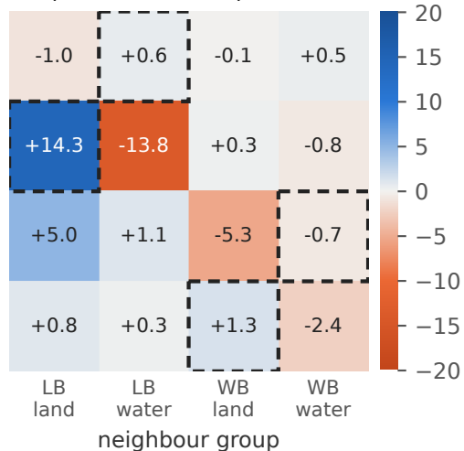
CoSpRo – raw CLIP (points)
