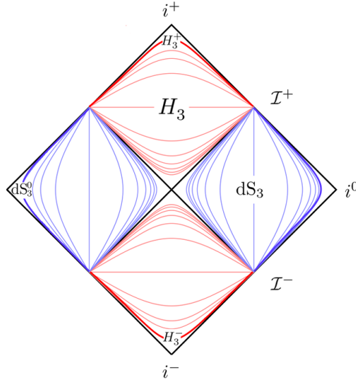
Figure 4: Penrose diagram of hyperbolic slicing of Minkowski space. The slices correspond to surfaces of constant \tau . The slices in the past and future lightcones of the origin have the geometry of H_3 , and the slices with spacelike separation from the origin have the geometry of dS_3 .
