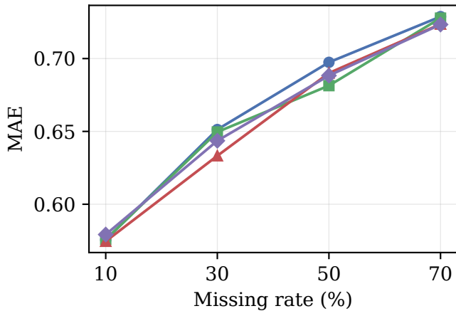
(b) MAE vs. missing rate
