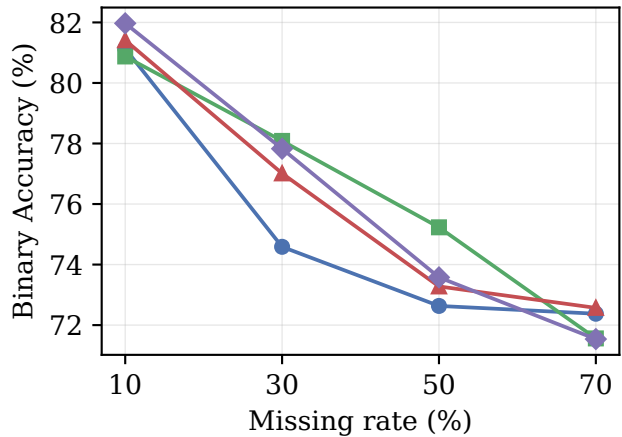
(a) Accuracy vs. missing rate
