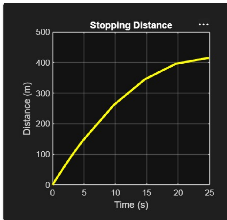
Figure 4: Cumulative stopping distance over time, illustrating deceleration curvature flattening as the train approaches rest at ~415 meters.
