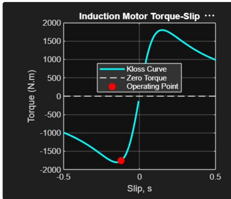
Figure 2: Electrodynamic torque-slip characteristic curve (Kloss formulation) indicating the stable regenerative braking quadrant ( s < 0 ) and operating point at s = -0.12 .
