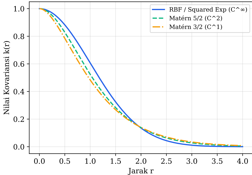
(a) Profil Kovariansi vs Jarak r = ||x - x'||
