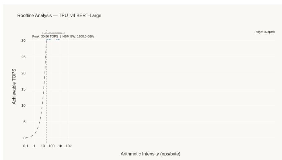
Figure 40: Roofline analysis for BERT-Large on TPU v4.
