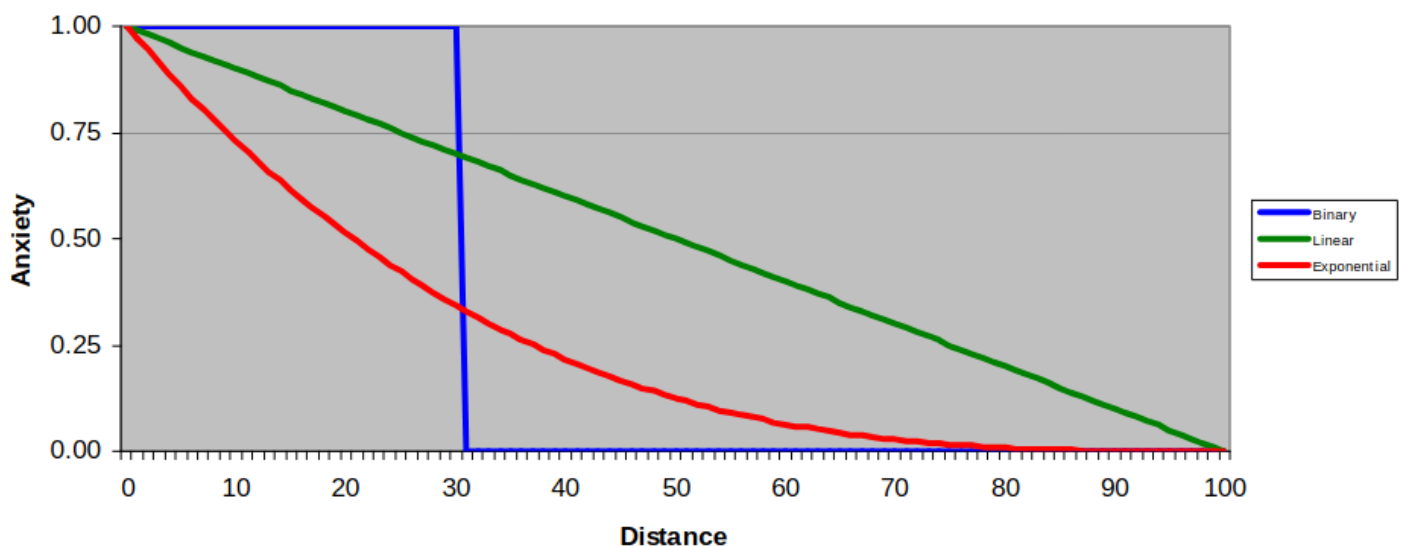
Exponential Threshold
