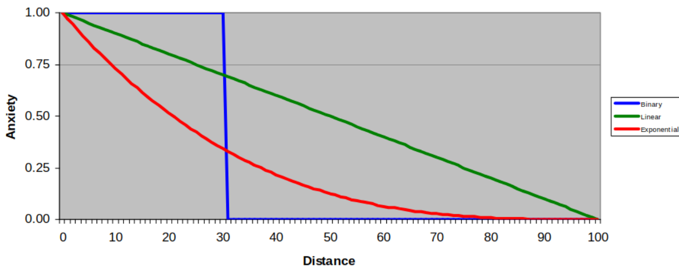
Exponential Threshold
