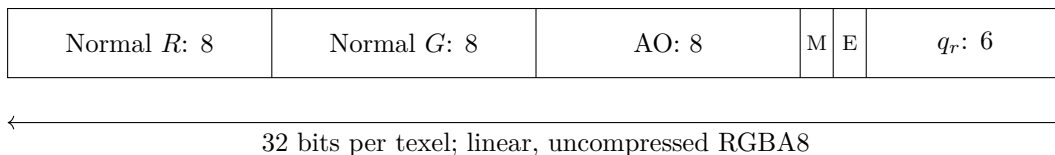
Figure 2: Surface texel layout. Metallic and emissive are flags, not continuous-valued material channels. Bit positions 7, 6, and 5–0 refer to the alpha byte.
