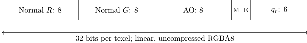
Figure 2: Surface texel layout. Metallic and emissive are flags, not continuous-valued material channels. Bit positions 7, 6, and 5–0 refer to the alpha byte.
