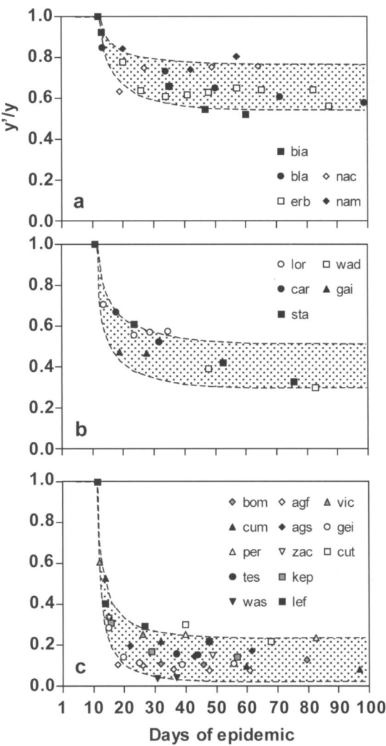
Fig. 5. Comparison between the relative contribution of primary downy mildew lesions to total lesions (ratio y'/y ) simulated by the model and observed in 23 vineyards with epidemics characterized by low (a), intermediate (b), and high (c) level of clonality. The lower and upper curves in each panel indicate the predicted outcome (shaded area) using 99% confidence intervals for the parameters Q , Pf , and R . These values were: (a) Q = 18,000 , Pf = 0.16 , R = 4.2 (lower curve), Q = 32,000 , Pf = 0.20 , R = 9.5 (upper curve); (b) Q = 1300 , Pf = 0.28 , R = 4.2 (lower curve), Q = 2,900 , Pf = 0.34 , R = 15.1 (upper curve); (c) Q = 300 , Pf = 0.41 , R = 16.4 (lower curve), Q = 400 , Pf = 0.49 , R = 22.6 (upper curve). Points are the real data collected in the vineyards (see Table 2 for vineyard characteristics).
