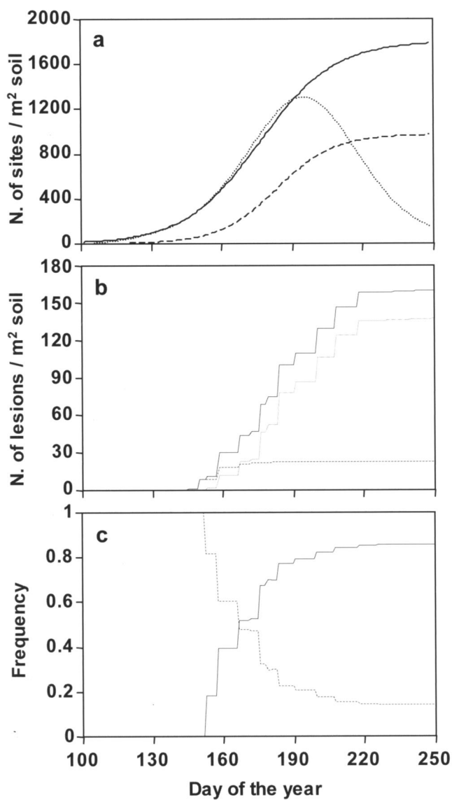
Fig. 2. Examples of model output: a, carrying capacity for Plasmopara viticola infections of the grapevine canopy, expressed as total number of sites in leaves on main (—) and lateral (---) shoots, and sites receptive to infection (····); b, number of primary oospore-derived (---), secondary clonal (····), and total (—) downy mildew lesions; c, proportion of the primary (---) and secondary (—) lesions over the total lesions.
