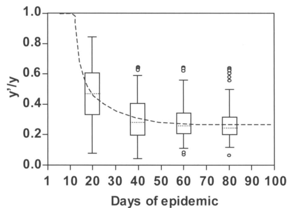
Fig. 4. Relative contribution of primary downy mildew lesions to total lesions (ratio y'/y ) simulated by the model. The model was operated 500 times by changing initial conditions and model parameters within a range of biologically plausible values. The line (---) is the average of the 500 simulations; the box plots show the data distribution at 20, 40, 60, and 80 days of the simulated epidemics. The box includes 50% of the data, the segment (--) is the median, the whiskers extend to maximum and minimum values, while points are outliers.
