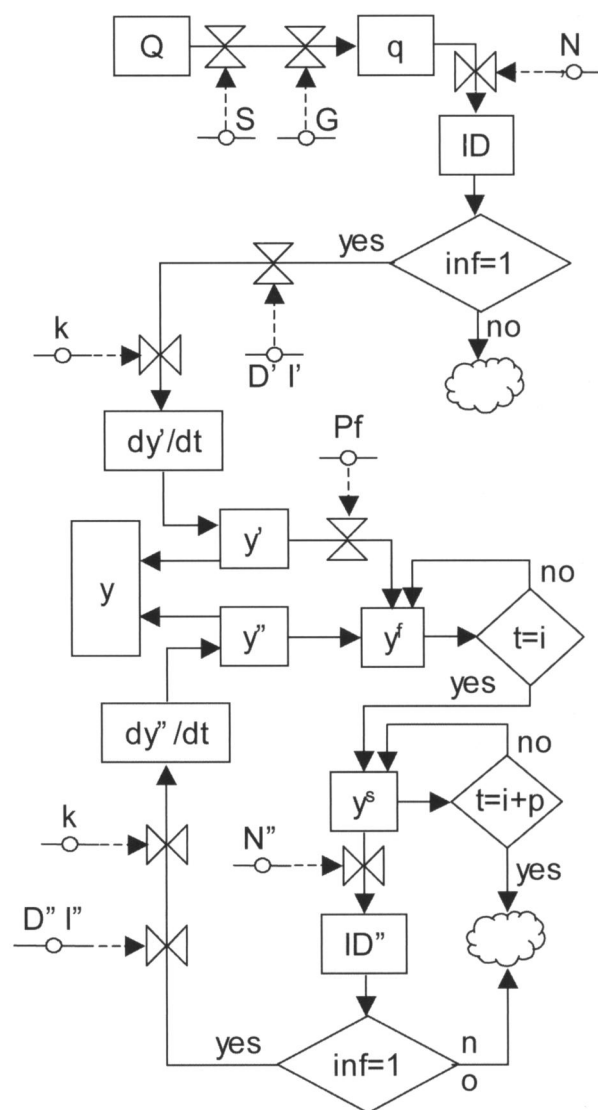
Fig. 1. Relational diagram of the model predicting primary and secondary infection cycles of Plasmodium viticola . Legend: □ state variable; → flux and direction of states; → flux and direction of information; ○ parameter; ◇ switch; ⊙ outgoing variable; ⊞ valve in a flux (rate) (see Table 1 for acronym explanations); inf is a dichotomic variable, with values 1 when there is infection and 0 when there is no infection.
