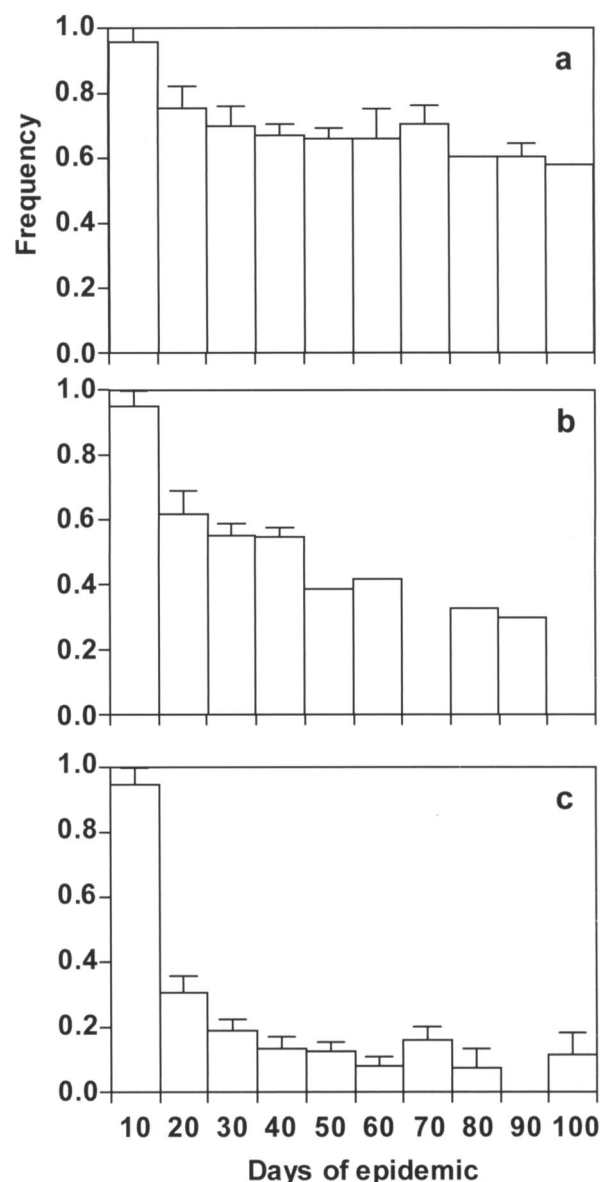
Fig. 3. Proportion of the downy mildew lesions caused by singleton Plasmopara viticola genotypes over total lesions in 23 vineyards with epidemics characterized by low (a), intermediate (b), and high (c) level of clonality (see Table 2 for vineyard characteristics). Bars are averages of 5 (a), 5 (b), and 13 (c) vineyards, and whiskers are the standard errors.
