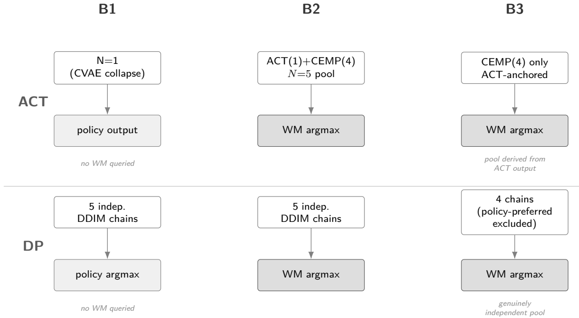
Figure 4.3 Three-branch evaluation framework for both policy families. B1 uses policy-internal selection only. B2 and B3 introduce world-model scoring; B3 excludes the policy’s preferred output. For DP the five candidates are structurally independent; for ACT, CEMP candidates are perturbations anchored to the single collapsed output.
