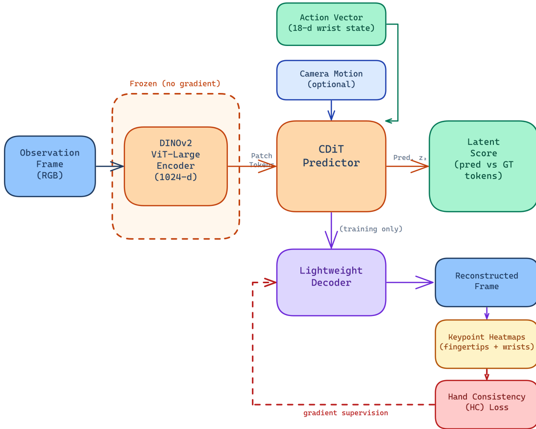
Figure 4.2 DexWM pipeline as implemented: frozen DINOv2 ViT-Large encoder producing spatial patch tokens; CDiT predictor conditioned on action and camera-motion inputs; lightweight decoder producing reconstructed frames and keypoint heatmaps; Hand Consistency (HC) loss supervising fingertip and wrist heatmap predictions during training. Latent score is computed by comparing predicted tokens against ground-truth tokens from the next frame. Adapted from [33].
