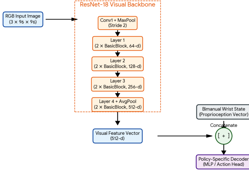
Figure 4.1 Shared ResNet-18 visual backbone used by both policy families. The backbone processes a single RGB frame ( 96 \times 96 pixels) through four residual stages (64, 128, 256, and 512 channels) and produces a 512-dimensional feature vector. This vector is concatenated with the bimanual wrist state proprioception vector before being passed to the policy-specific decoder. Adapted from [47].
