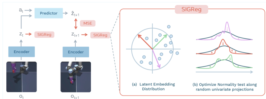
Figure 3.9 LeWM training pipeline: encoder, dynamics predictor, and SIGReg regulariser [26].
