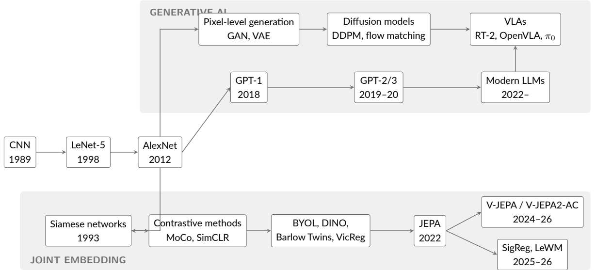
Figure 3.3 The post-AlexNet split of visual representation learning into a generative branch, culminating in diffusion models and the VLAs debated above, and a joint-embedding branch, culminating in JEPA-style latent world models including the families evaluated in this benchmark. Adapted from [41].
