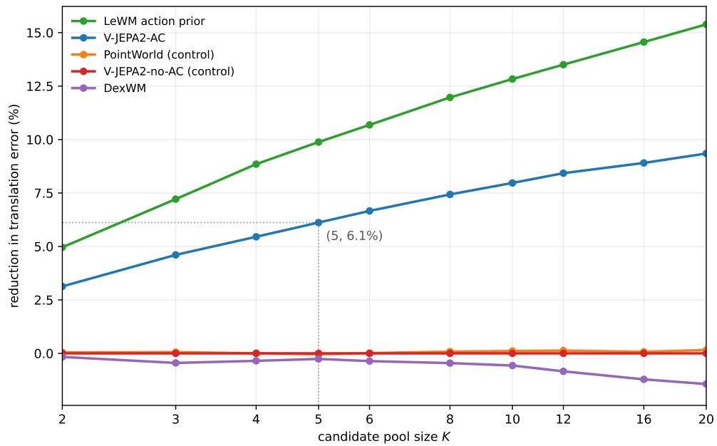
Figure B.3 Reduction in translation error against candidate pool size for the five world-model scorers on the Diffusion Policy row. All points are scored on nested pools, so differences along a curve reflect pool size alone. Pooled across 3 seeds except DexWM, which remains single-seed (Section 4.7). The vertical guide marks the operating point used throughout this dissertation.
