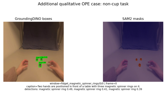
Figure 6: Additional qualitative Object Pose Estimation (OPE) pipeline example from a ring handling episode, included to show a second object configuration beyond the cup dominated case.
