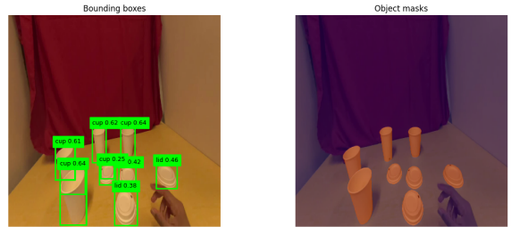
Figure 5: Example placement output from the grounding and mask stages. Semantic object prompts become bounding boxes and binary masks for the sampled window frames.
