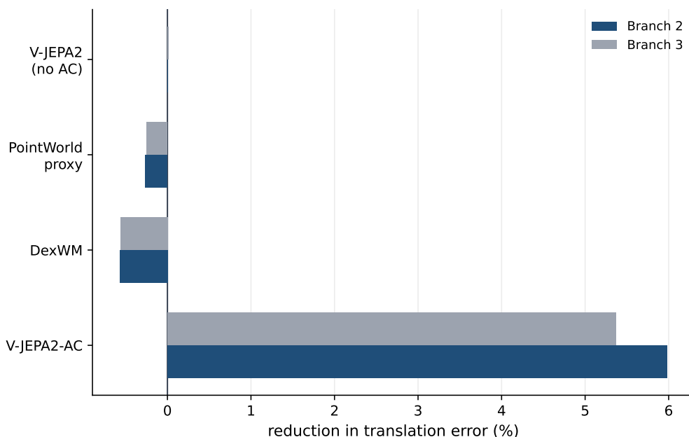
Figure 6.1 Reduction in translation error against the frozen DP candidate-0 baseline, by world model and branch. Positive values are an improvement over the policy-only candidate. Values are pooled across three training seeds except DexWM, which remains single-seed (Section 4.7).
