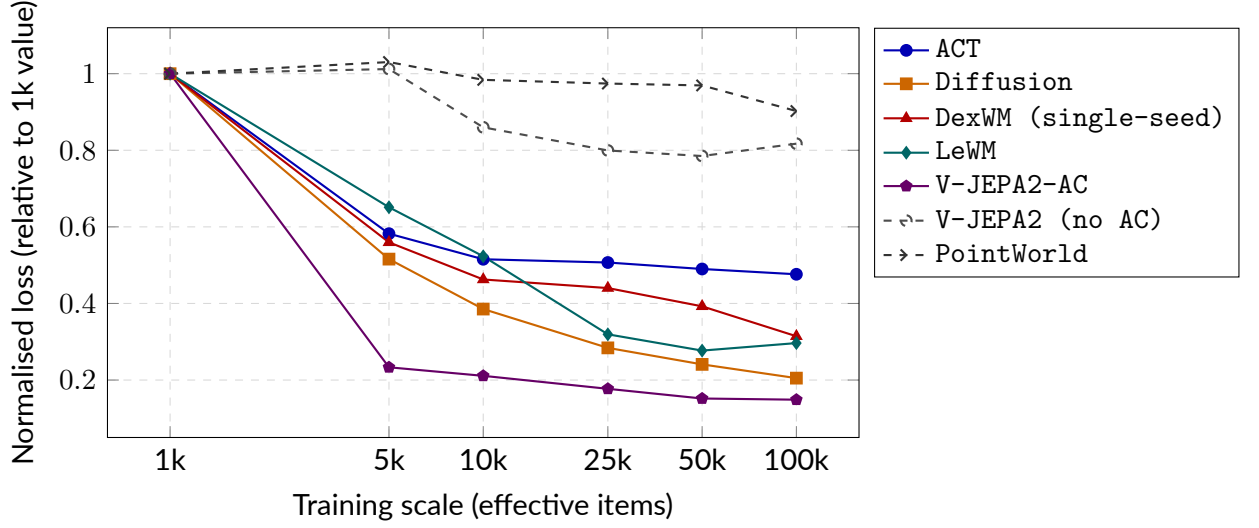
Figure B.3 Normalised validation loss (each family's value divided by its 1k loss) across six training scales, pooled across 3 seeds except DexWM (single-seed). Solid lines are primary models; dashed lines are controls.
