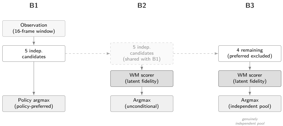
Figure 4.2 Three-branch evaluation framework (Section 4.2), shown for a policy producing five independent candidates. B2 and B3 reuse the same candidate pool generated for B1, relayed through the branches (dashed lines) rather than regenerated; B3 additionally removes the policy’s preferred candidate before scoring. Both ACT and DP follow this design; the per-policy candidate-generation mechanics are detailed in Section 4.3.
