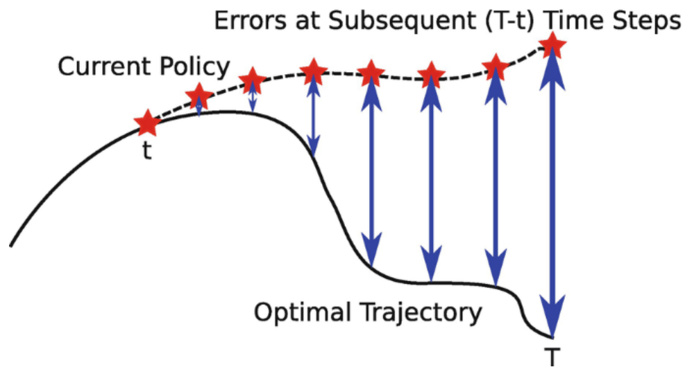
Figure 2.3 Compounding error in behaviour cloning. The policy trajectory drifts progressively further away at each step. The growing gap between the two paths illustrates how small errors can accumulate over time [14].
