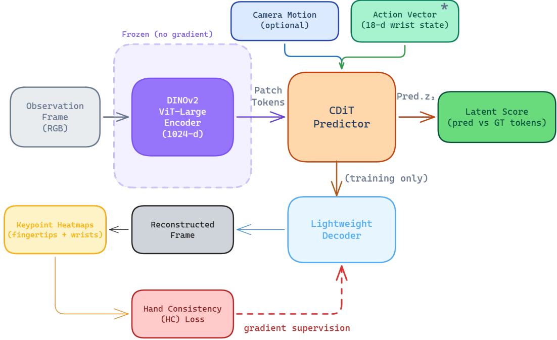
Figure 5.8 DexWM pipeline as implemented, comprising a frozen DINOv2 encoder, CDiT predictor, lightweight decoder, and HC loss supervision path. Adapted from [23].
