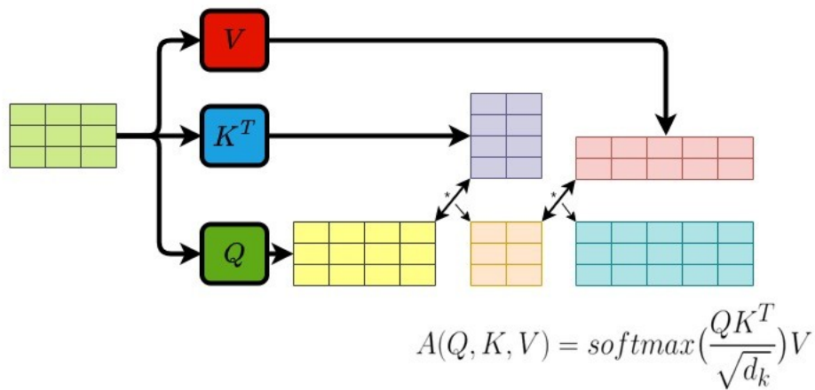
Figure 2.9 Transformer attention block: each token queries all others with Q , gathers weighted values V via keys K , and the weighted sum yields the updated output token [21].
