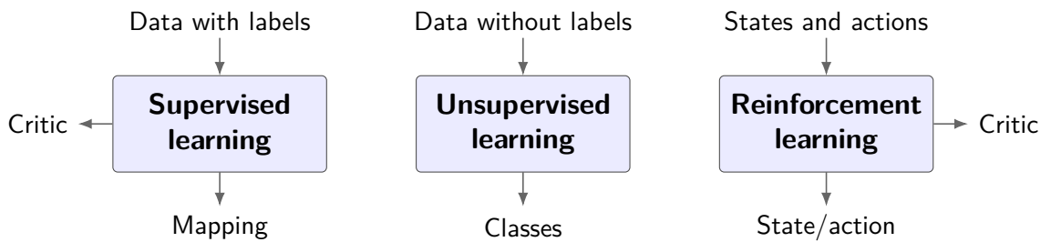
Figure 2.1 The three classical machine learning paradigms: supervised learning trains on labelled data, unsupervised learning extracts structure from unlabelled data, and reinforcement learning learns from a reward signal over states and actions [12]. SSL, central to the world models in this work, is a modern form of learning from unlabelled data in which prediction targets are constructed from the data itself [13].
