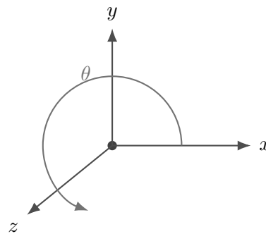
Figure 2.5 Rotation of the wrist about the y -axis by angle \theta ; the same construction applies about x and z , and the wrist's full orientation is the combined rotation about all three, represented as a rotation matrix R \in SO(3) [15].
