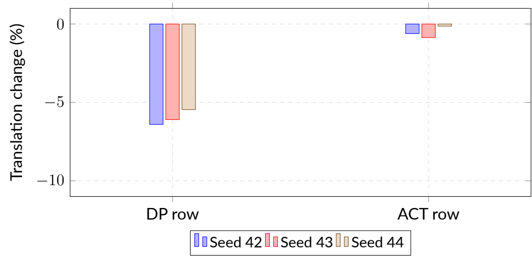
Figure 6.2 V-JEPA2-AC’s Branch 2 translation change across three training seeds, DP row and ACT row. Level bars indicate a stable result; the DP row’s three bars sit close together, confirming the headline result is not a single-run artefact.
